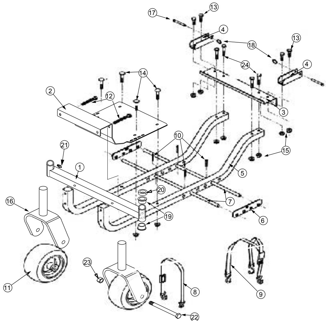
Fig. 1. JRCO Blower Buggy™ Carrier Parts Drawing
