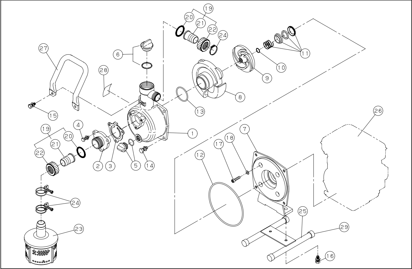
DWG No.012883201 MODEL:SEH-25L FORM:SEH-25L-BAA-0
