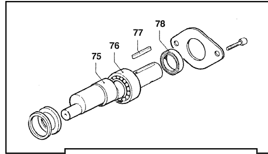
Version with 30mm solid shaft
